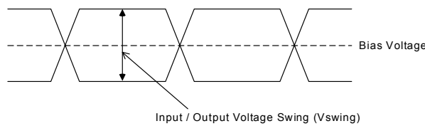
Figure 6. Definition of differential input/output voltage swing
