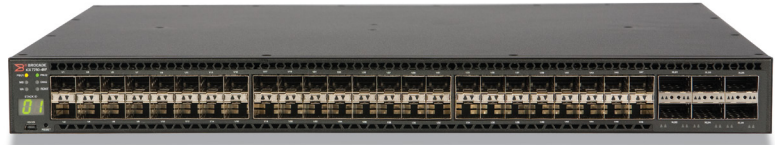
Figure 1. The Brocade ICX 7750-48F features 48 1/10 GbE SFP+ ports and 6 40 GbE QSFP+ ports that can each be split into 4×10 GbE SFP+ ports. The front panel also displays the unit stacking ID.
