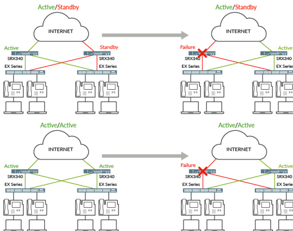
Figure 2: High availability
