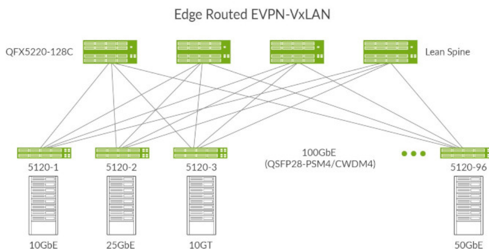
Figure 3: Private cloud data center with the QFX5220-128C as lean spine
