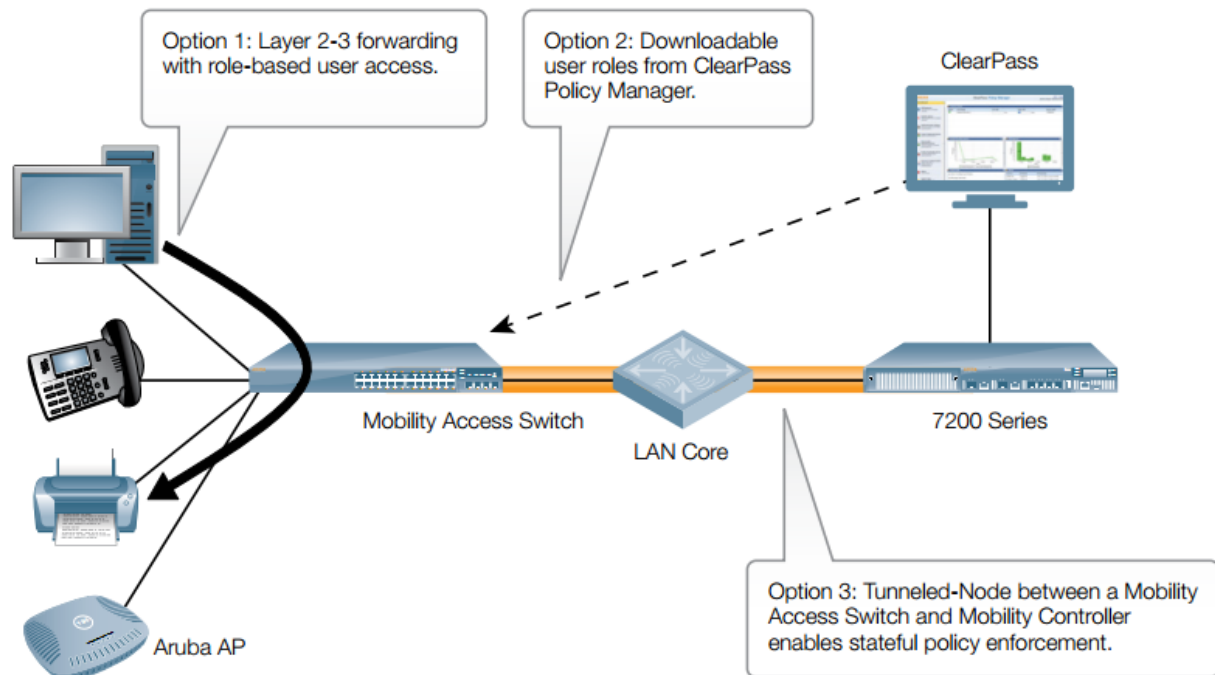
Figure 1. Flexible secure wired access deployments
