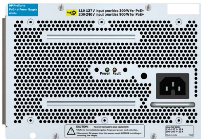
Figure 3. The J9306A - z1 1500W PoE+ Power Supply
