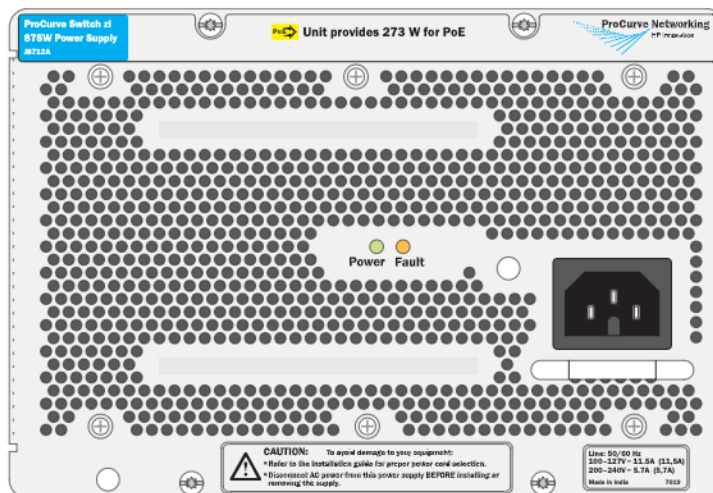
Figure 1. The J8712A - zl 875W PoE Power Supply
