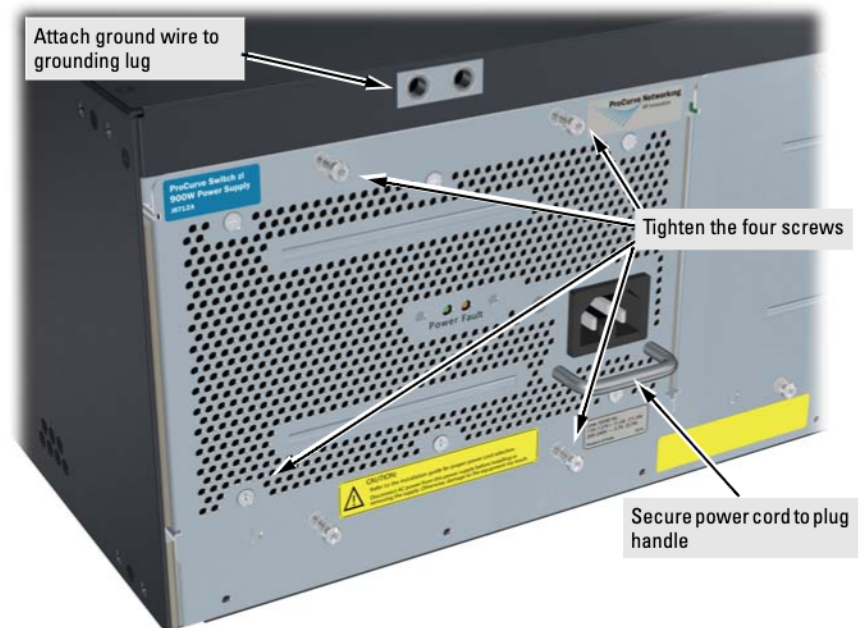
Figure 5. Fully installed power supply
