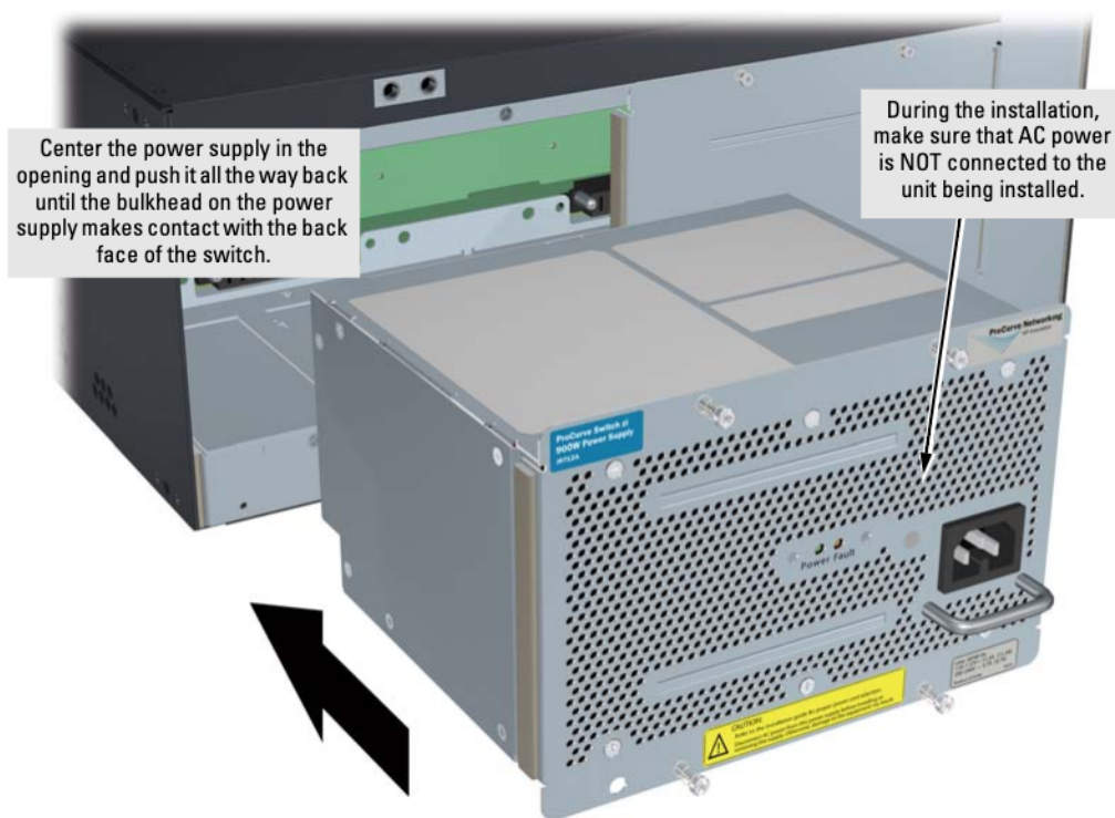
Figure 4. Installing a power supply
