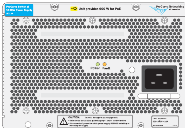
Figure 2. The J8713A - zl 1500W PoE Power Supply
