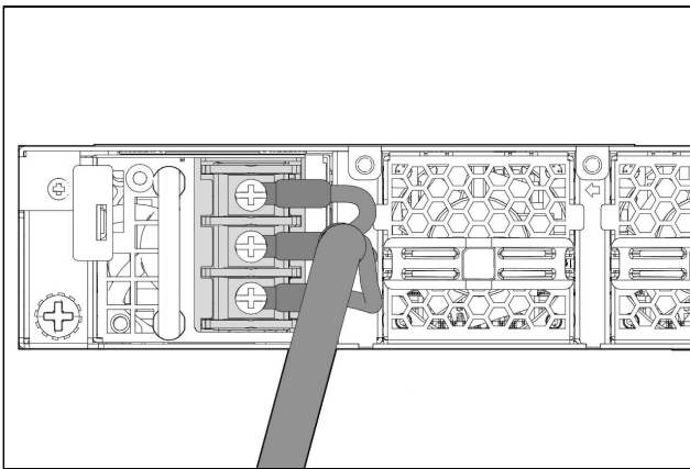
Figure 16 Connecting DC Power to the Switch
