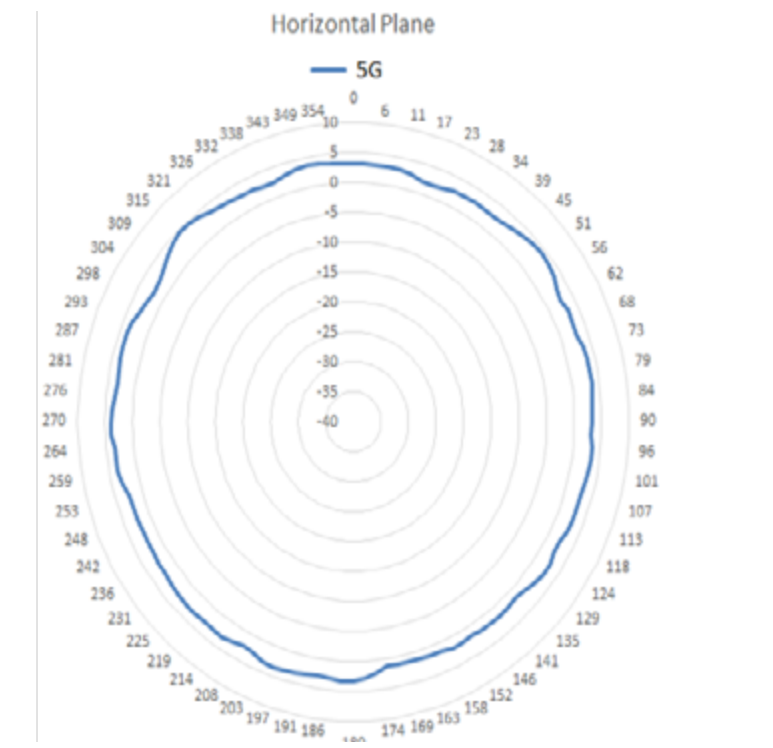
AP505i Antenna Radiation Patterns — 5.0GHz
