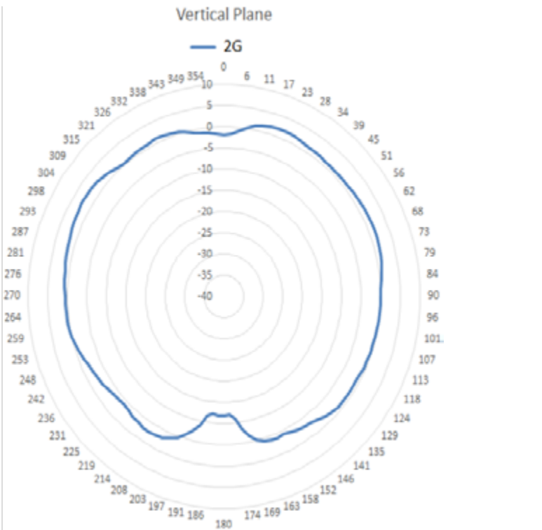
AP505i Antenna Radiation Patterns — 2.4GHz
