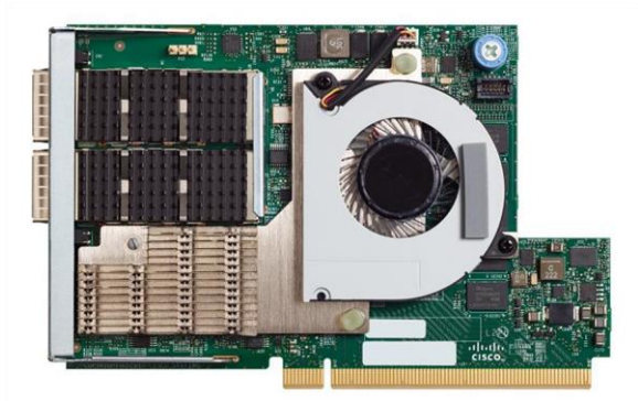
Figure 20. Cisco UCS VIC 1497
