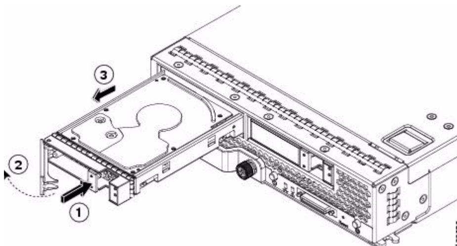
Figure 1-13 Removing the Drive
