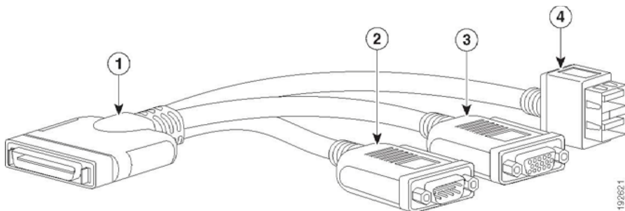
Figure 14 KVM Cable
