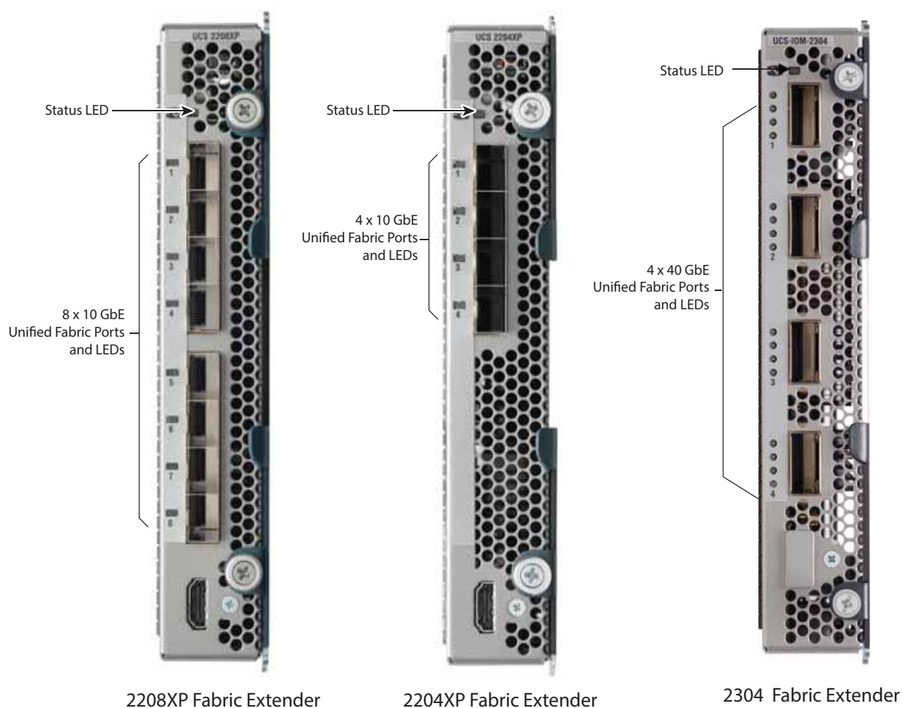
Figure 7 2208XP, 2204XP, and 2304 Fabric Extender
