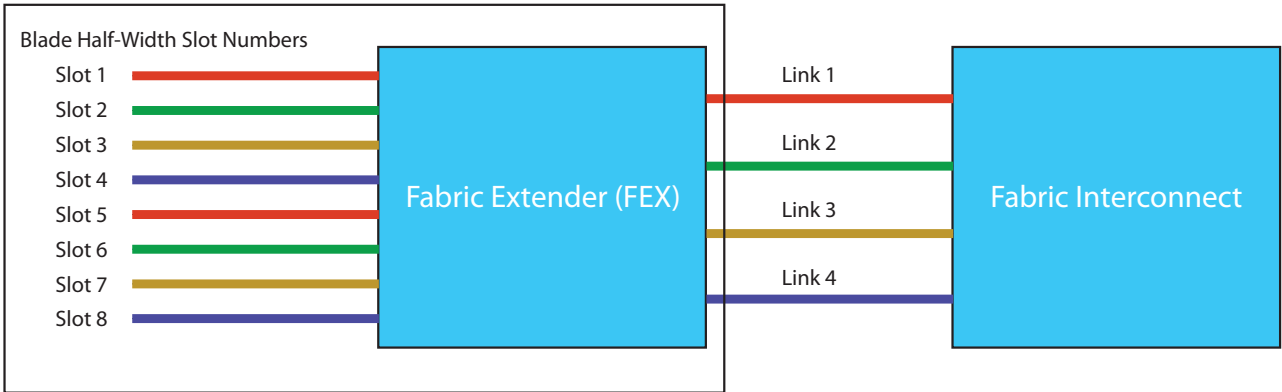
Figure 12 Discrete Mode FEX Fabric Link Blade Chassis
