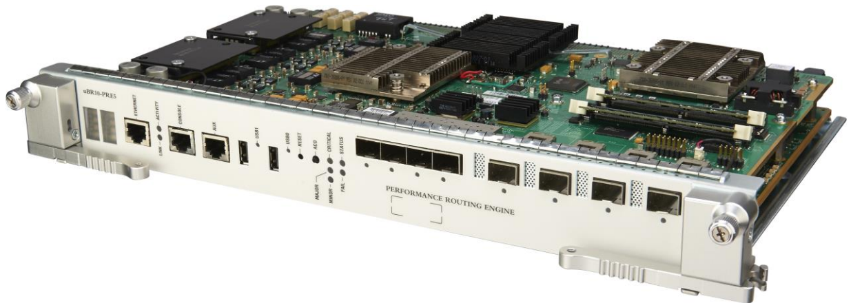
Figure 1. Cisco uBR10012 Performance Routing Engine 5 (UBR10-PRE5) for the Cisco uBR10012 Universal Broadband Router
