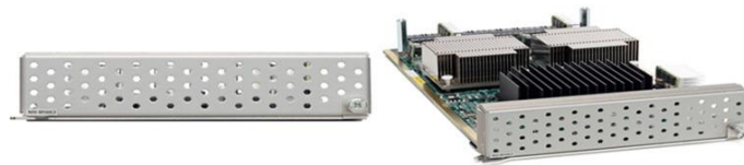
Figure 8. Layer 3 Module (Front View and Side View)
