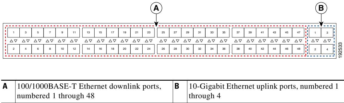
Figure 3-3 Port Numbering on the Cisco Nexus 2248TP-E FEX
