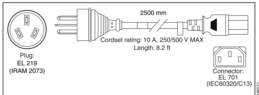
Figure C-1 SFS-250V-10A-AR
