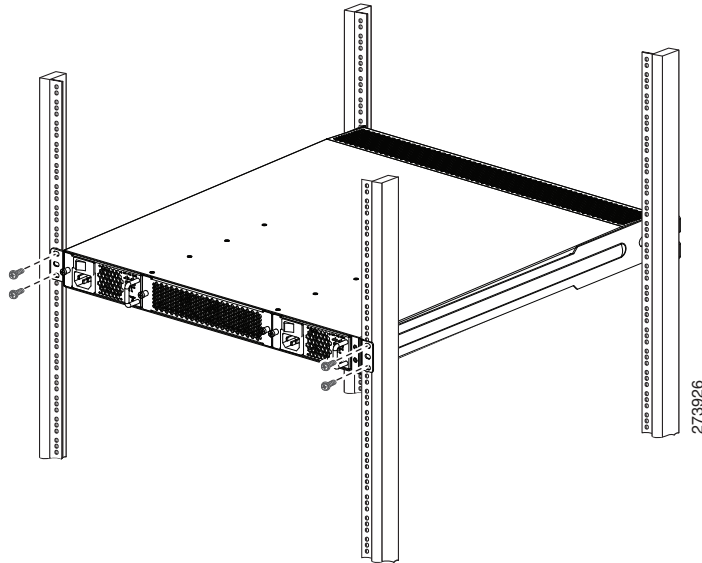
Figure 4-4 Attaching the Device to the Rack
