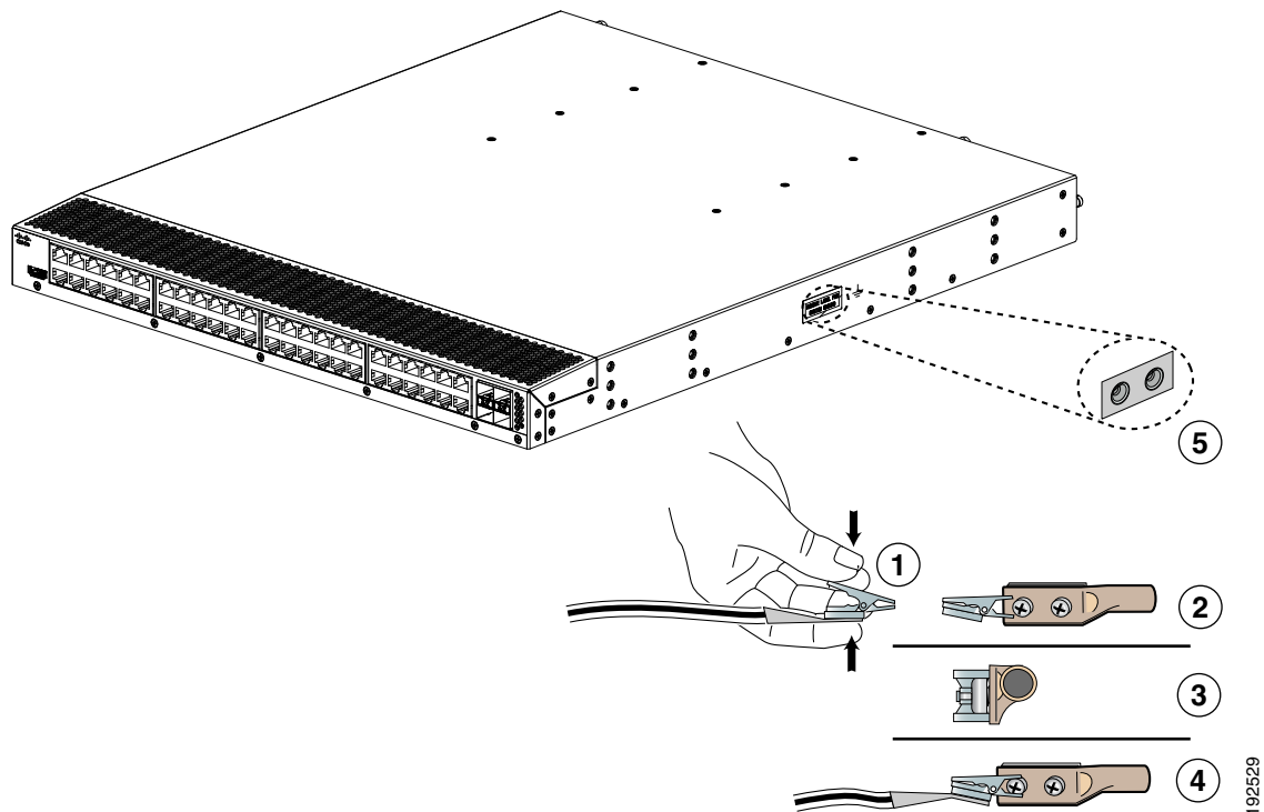
Figure 4-5 Attaching the ESD Wrist Strap to the System Ground Lug Screw
