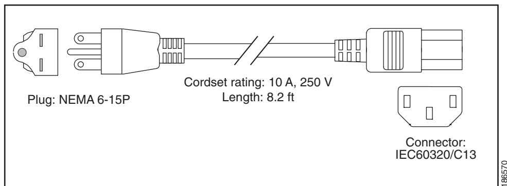
Figure C-11 CAB-N5K6A-NA
