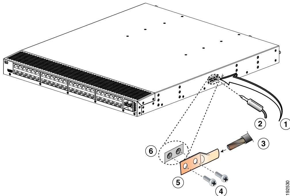
Figure 4-6 Location of System Ground on a Cisco Nexus 2000 Series FEX
