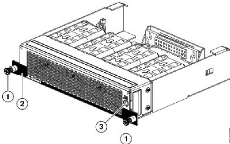
Figure 3-20 Back-to-Front Airflow Fan Tray for the Cisco Nexus 2232PP and 2232TM FEXs
