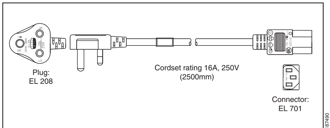
Figure C-5 SFS-250V-10A-ID
