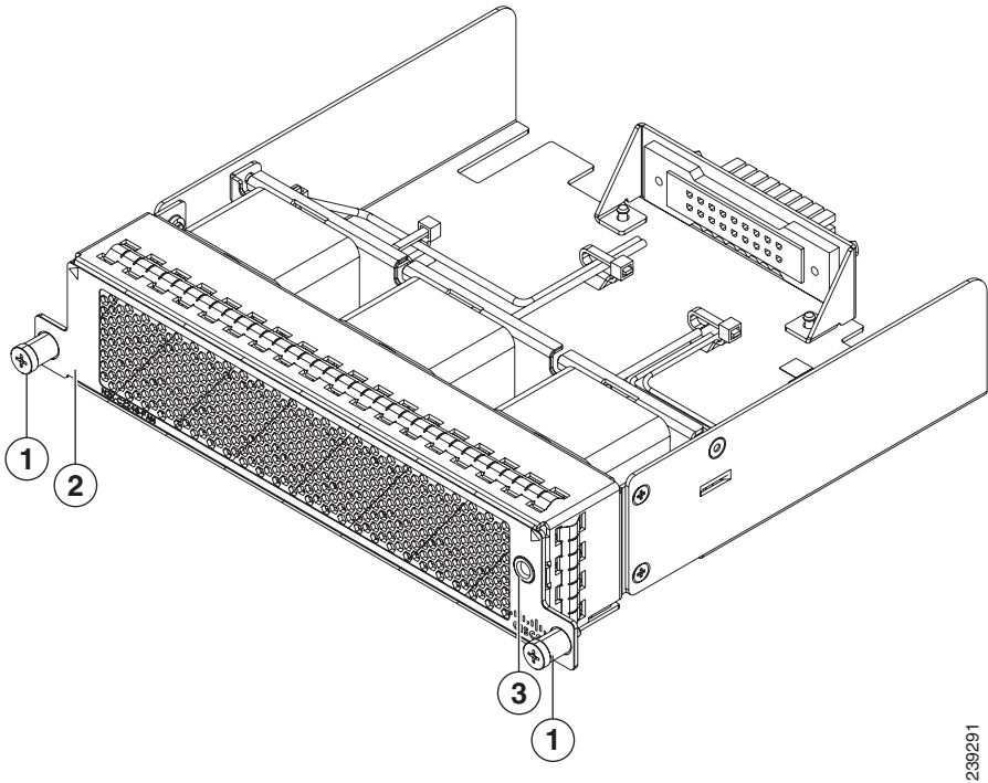
Figure 2-8 Front-to-Back Airflow Fan Tray for the Cisco Nexus 2000 Series FEX
