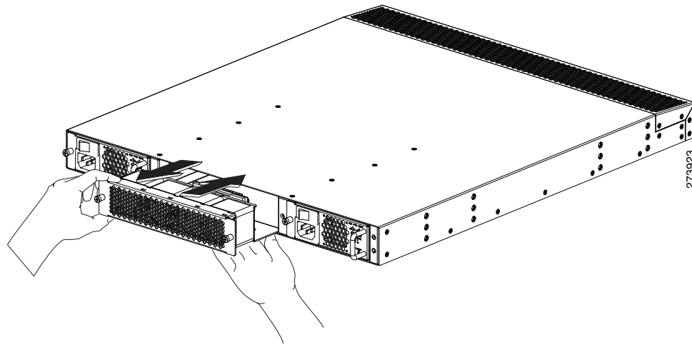
Figure 4-8 Fan Tray for the Cisco Nexus 2000 Series FEX
