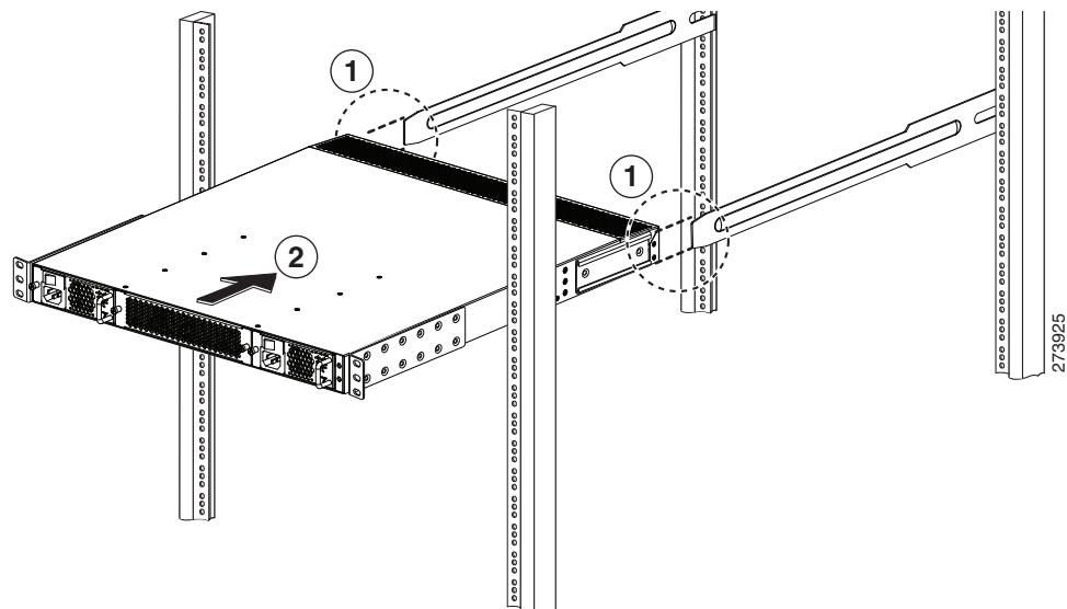
Figure 4-3 Sliding the Chassis Into the Rack
