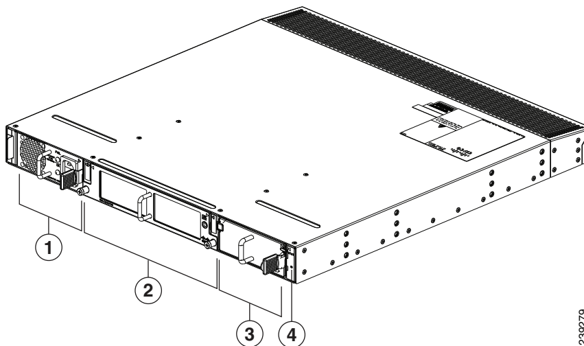
Figure 2-21 Front View of the Cisco Nexus 2232PP Chassis
