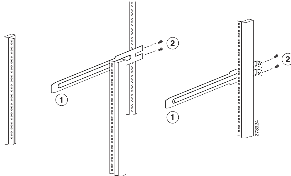
Figure 4-2 Installing the Slider Rails
