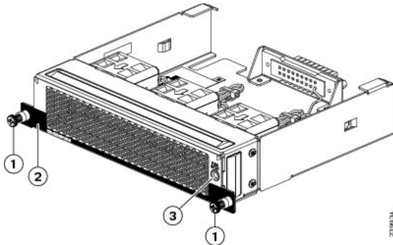
Figure 3-9 Back-to-Front Airflow Fan Tray for the Cisco Nexus 2000 Series FEX
