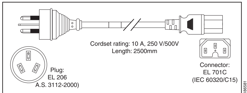
Figure C-2 CAB-9K10A-AU
