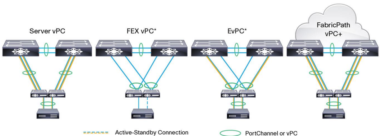
Figure 7. Cisco Nexus 2000 Series Fabric Extenders Design Scenarios, from Left to Right: Server vPC, FEX vPC, EvPC, vPC+
