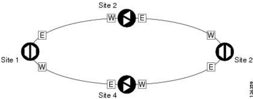
Figure 45: Hubs with Line Amplifiers
