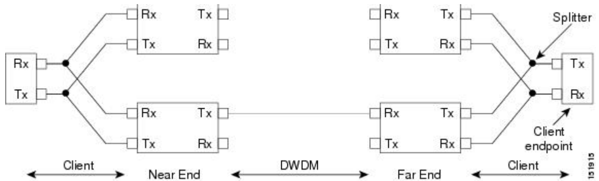
Figure 47: Y-Cable Protection
