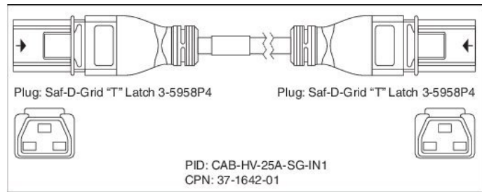
Figure 31: CAB-HV-25A-SG-IN1 Power Cord and Plugs for the 3.5-kW HVAC/HVDC Power Supply Unit
