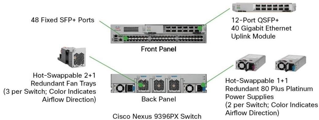
Figure 9. Cisco Nexus 9300 Platform Components
