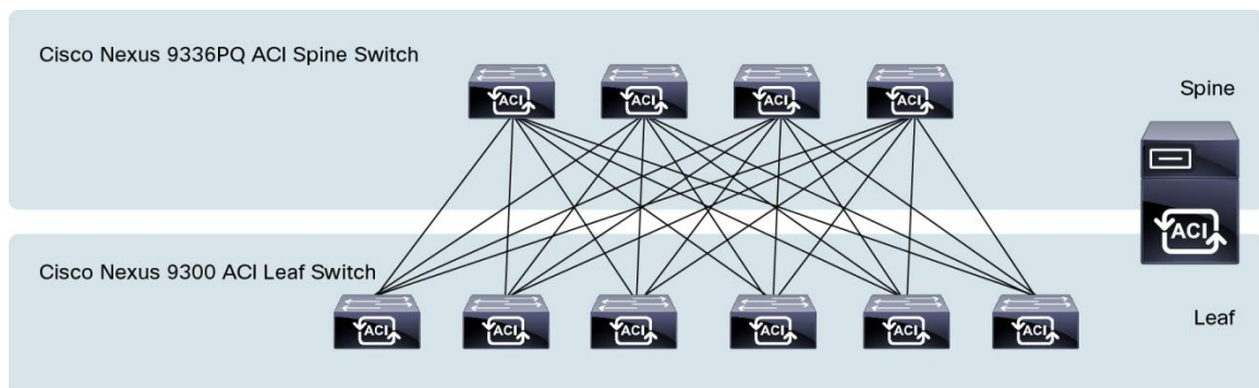
Figure 12. Cisco Nexus 9300 Platform Leaf-and-Spine Architecture for Cisco ACI
