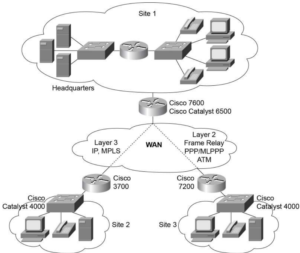
Figure 2. WAN Aggregation
