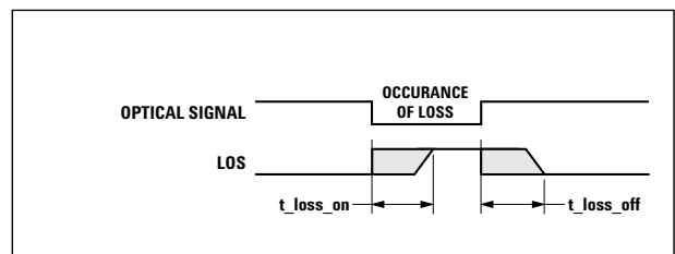
t-los-on & t-los-off
