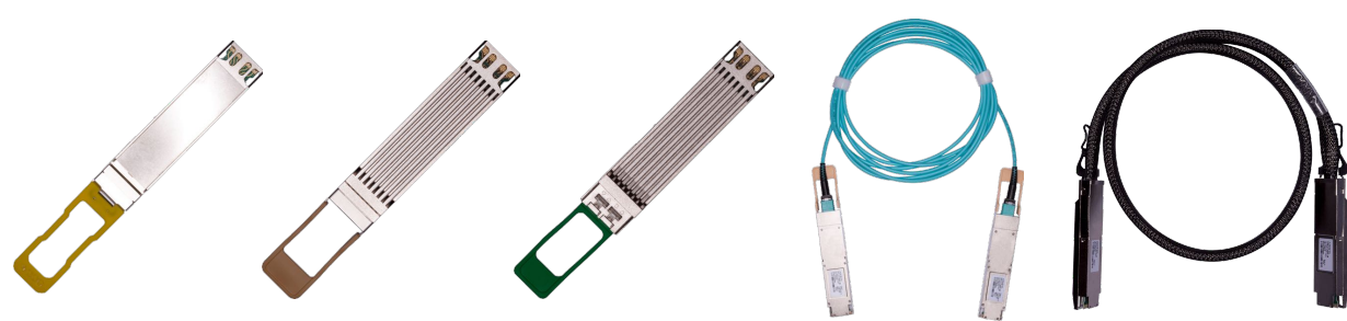
Broad portfolio of Arista 400G OSFP and QSFP-DD optics, AOCs and copper DACs
