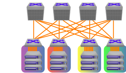
Arista Leaf-Spine Two-tier Network Architecture with 7060X and 7260X Series
