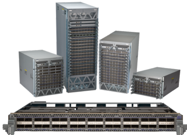
Arista 36 port 100GbE line card with MACsec for 7500R
