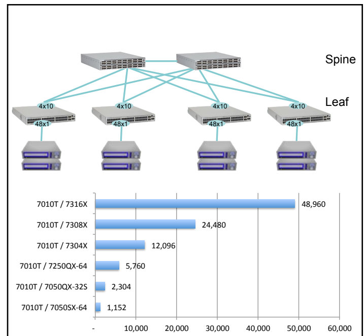
Arista Leaf-Spine Design with L2 MLAG all at 1.2:1
